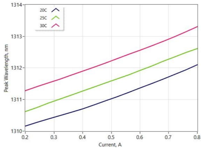
Peak Wavelength Tuning by Current
